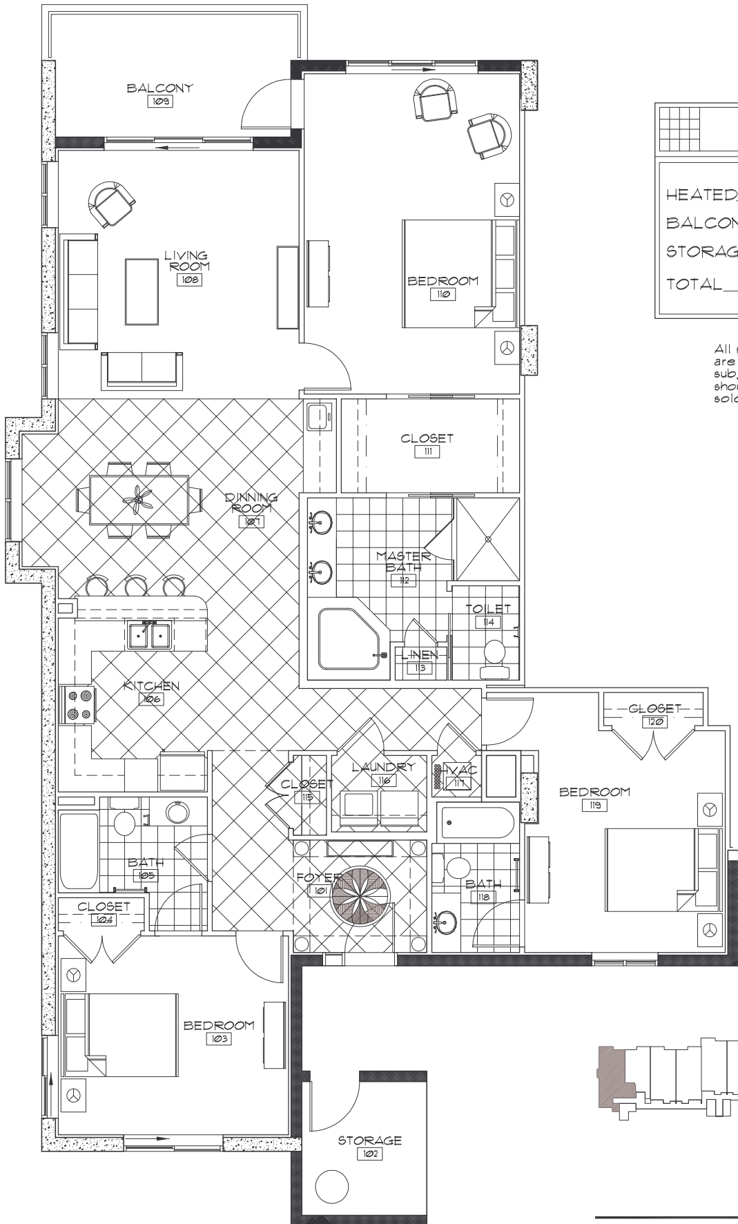
UNIT 'B' FLOOR PLAN
